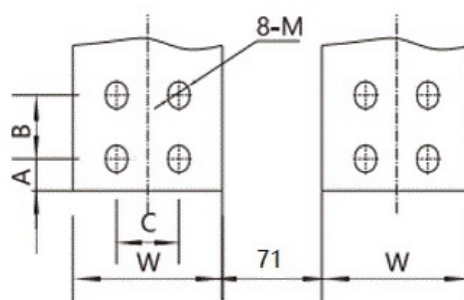
double-layer busway
